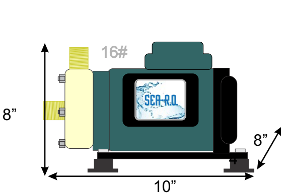
FEED PUMP
