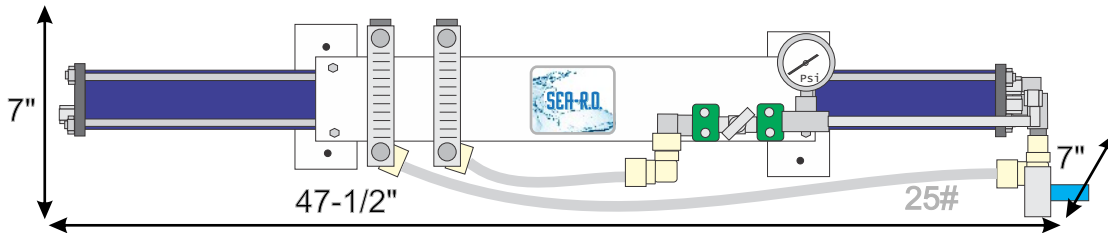
PRESSURE VESSEL ARRAY
