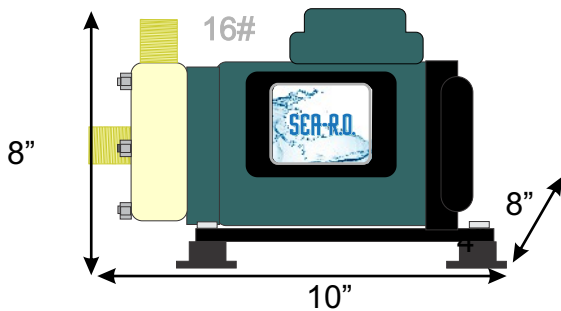
FEED PUMP
