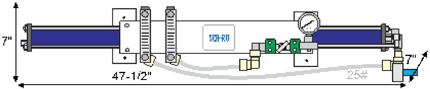
“Nautilus” 500 Membrane and Pressure Vessel Array
