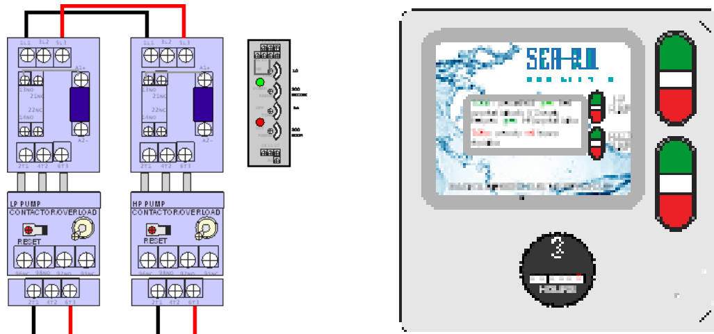
“Nautilus” System Control Panel
